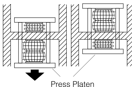
FORMING PRESS
