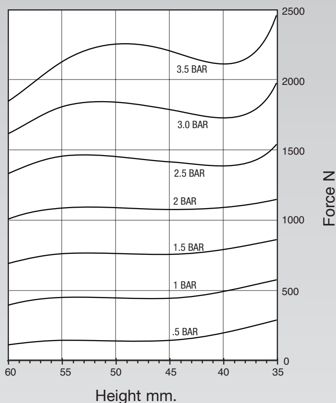
Force Table (Use for Airstroke™ actuator design)
