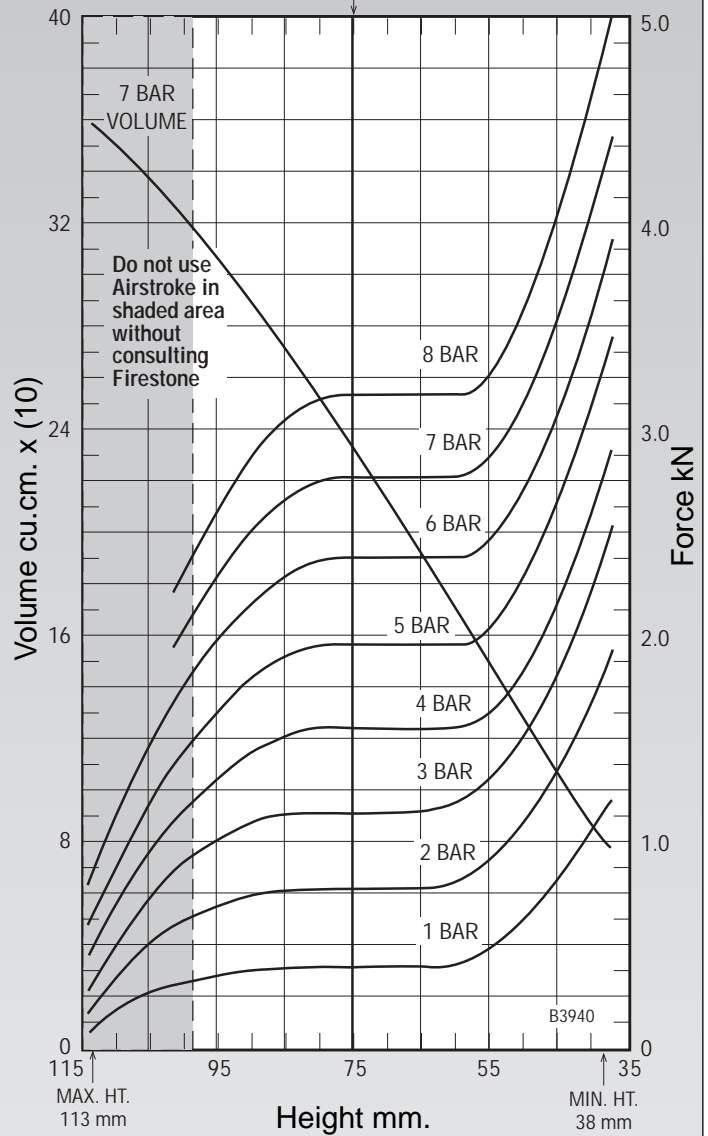
RECOMMENDED AIRMOUNT DESIGN HEIGHT 75 mm. Static Data A9618
