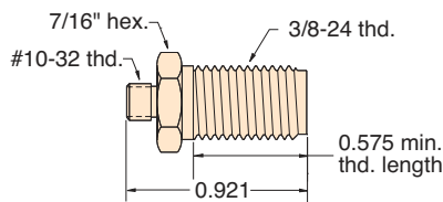
Part No. MJQC-VMT Description . . . . .#10-32 Male, 3/8-24 Thd. (supplied with mounting nut and two washers)
