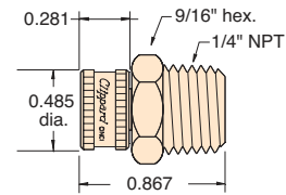
Part No. MJQC-CMQ Description . . . . .1/4" NPT
