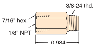
Part No. MJQC-VFP Description . . . . .1/8" NPT Female, 3/8-24 Thd.
