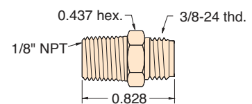
Part No. MJQC-VMP Description . . . . .1/8" NPT Male, 3/8-24 Thd.
