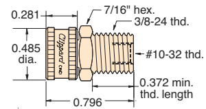
Part No. MJQC-CPF Description . . . . .3/8" Thread
