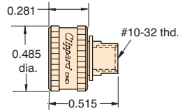
Part No. MJQC-CFT Description . . . . .#10-32
