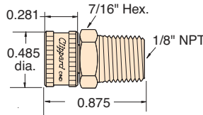
Part No. MJQC-CMP Description . . . . .1/8" NPT
