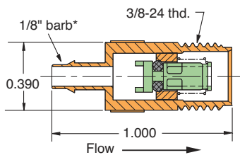
Part No. MJQC-VB4 Description . . . . .1/8" Barb, 3/8-24 Thd.
