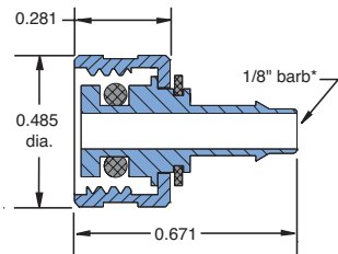
Part No. MJQC-CB4 Description . . . . .1/8" Barb
