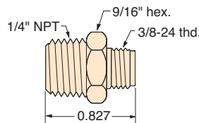
Part No. MJQC-VMQ Description . . . . .1/4" NPT Male, 3/8-24 Thd.
