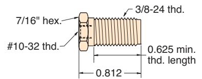
Part No. MJQC-VFT Description . . . . .#10-32 Female, 3/8-24 Thd. (supplied with mounting nut and two washers)
