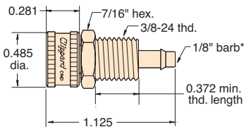
Part No. MJQC-CPB Description . . . . .1/8" Barb (supplied with mounting nut and two washers)
