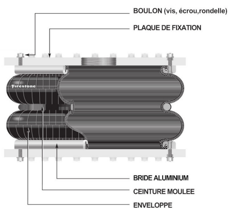
A brides aluminium Type D
