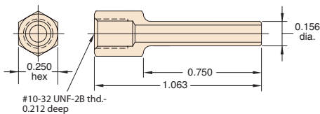
11675-05 5/32" OD Tube
