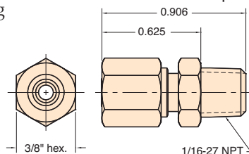
1/16" NPT to 1/8" O.D. Tube Compression Fitting
