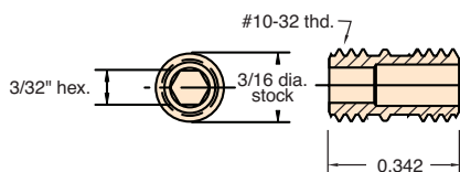
#10-32 Extension Fitting
