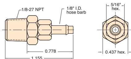
1/8" NPT to 1/8" I.D. Hose Swivel Fitting
